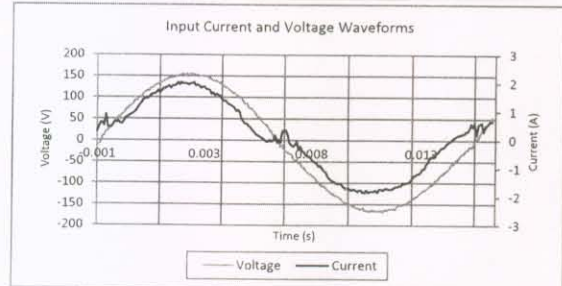
Input AC Current Waveform (ITHD = 14.646%, 50% Load)
