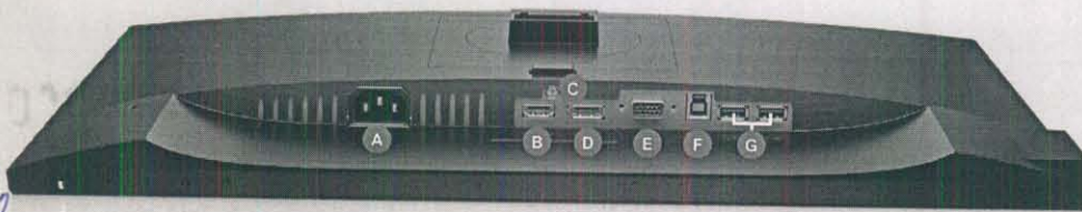
Back view - Cable management slot
