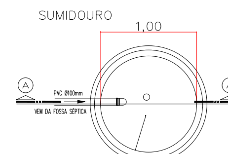
VISTA SUPERIOR esc: 1/40
