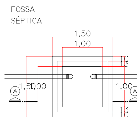
VISTA SUPERIOR esc: 1/40
