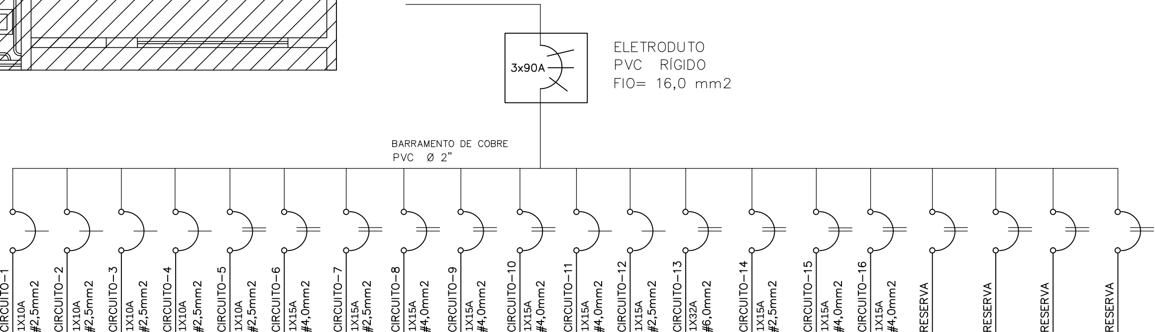
DIAGRAMA UNIFILAR
